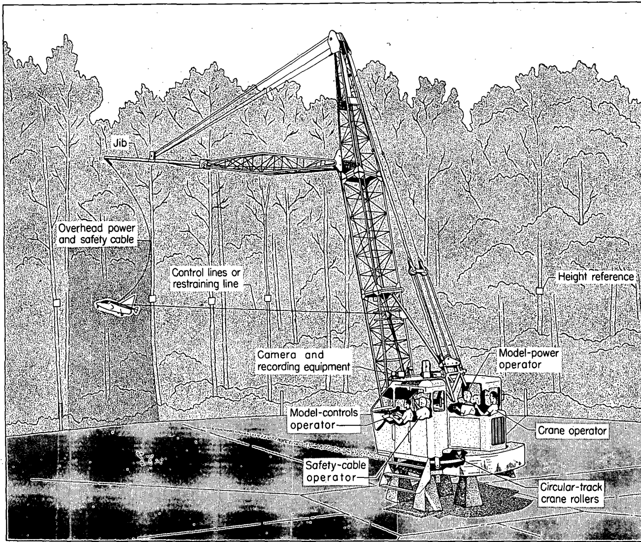
Figure 8.- The Langley control-line facility.
