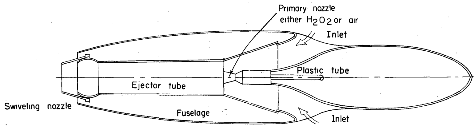
Figure 6.- Sketch of rocket motor installation inside the model.
