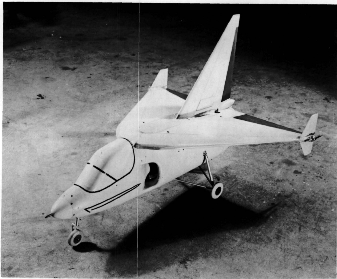
Figure 1.- Three-quarter front view of the 1/5-scale model of the Ryan X-13 VTOL airplane. L-94531
