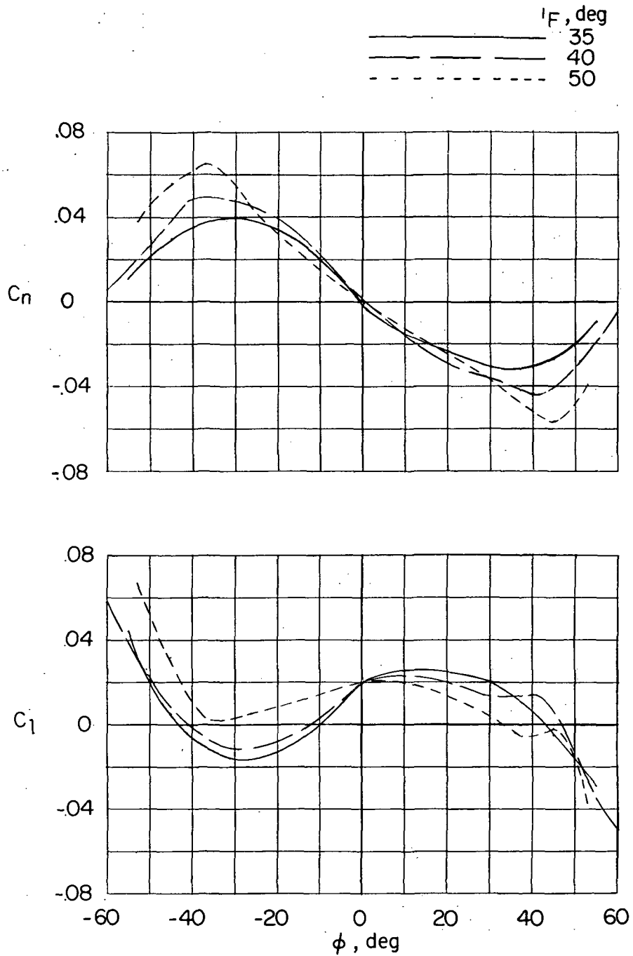
Figure 13.- Variation of C_l and C_n with \phi about the body axis for several angles of attack. \delta_e = -10^\circ , \delta_a = 0^\circ .
