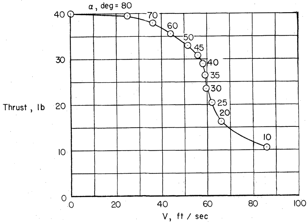
Figure 11.- Angle of attack and thrust required against airspeed for 1/5-scale model Ryan X-13 VTOL airplane.
