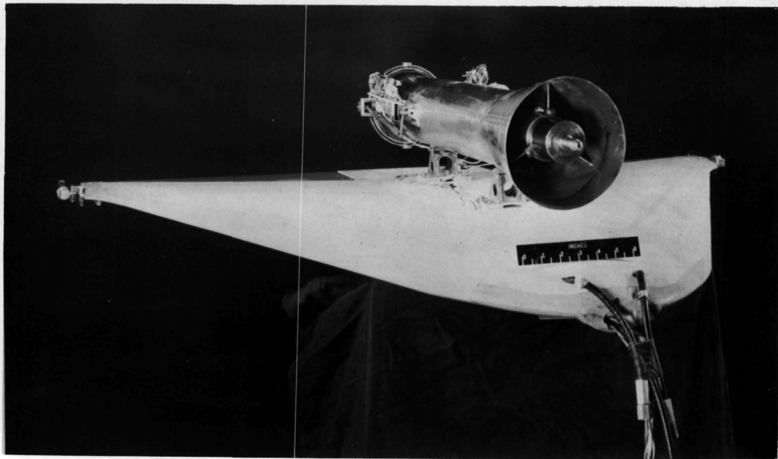
Figure 4.- Three-quarter front view of the hydrogen peroxide power plant used in the 1/5 -scale model of the Ryan X-13 VTOL airplane.
