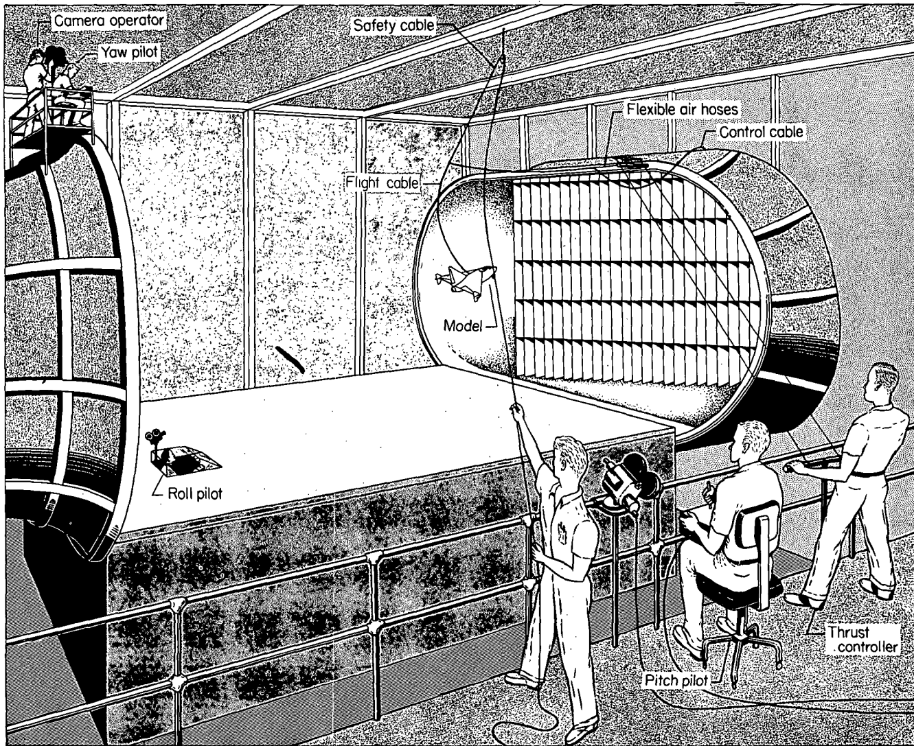
Figure 7.- Test setup for flight tests in the Langley full-scale tunnel.
