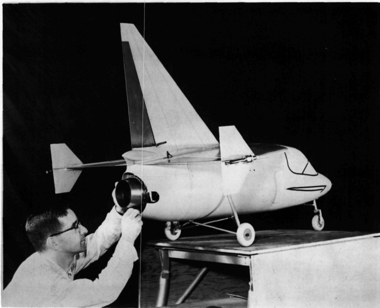
Figure 2.- Three-quarter rear view of the 1/5-scale model of the Ryan X-13 VTOL airplane.
