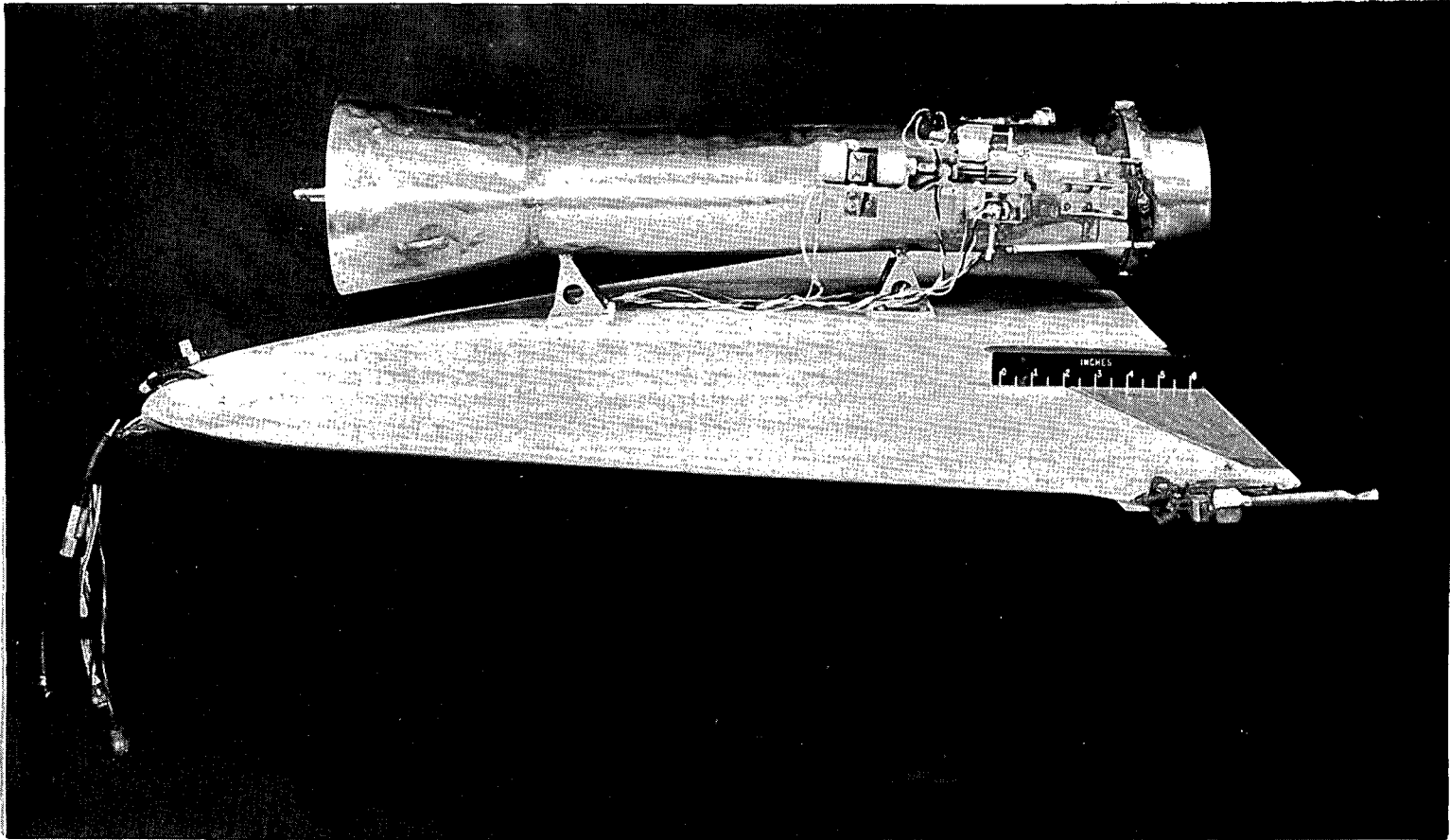
Figure 5.- Side view of the hydrogen peroxide power plant used in the 1/5-scale model of the Ryan X-13 VTOL airplane.
