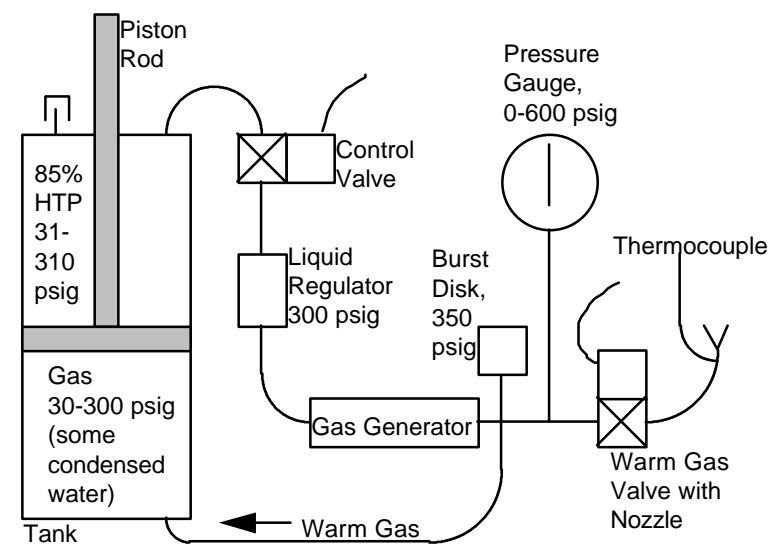
Figure 7. Self pressurizing HTP test system schematic.
