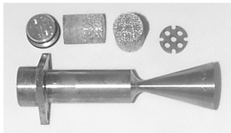
Figure 3. Monopropellant HTP thruster.
