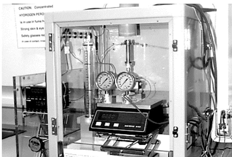
Figure 4. Thrust stand setup in benchtop safety enclosure.
