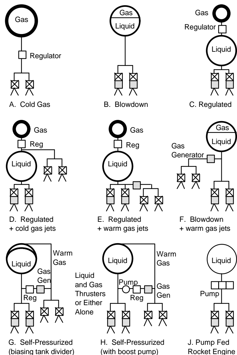
Figure 5. Simplified schematics of propulsion systems.
